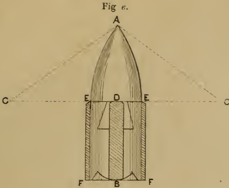
RIPLE BALL COMPLETE, WITH THE FORE- PART OF ZINC OR IRON,
